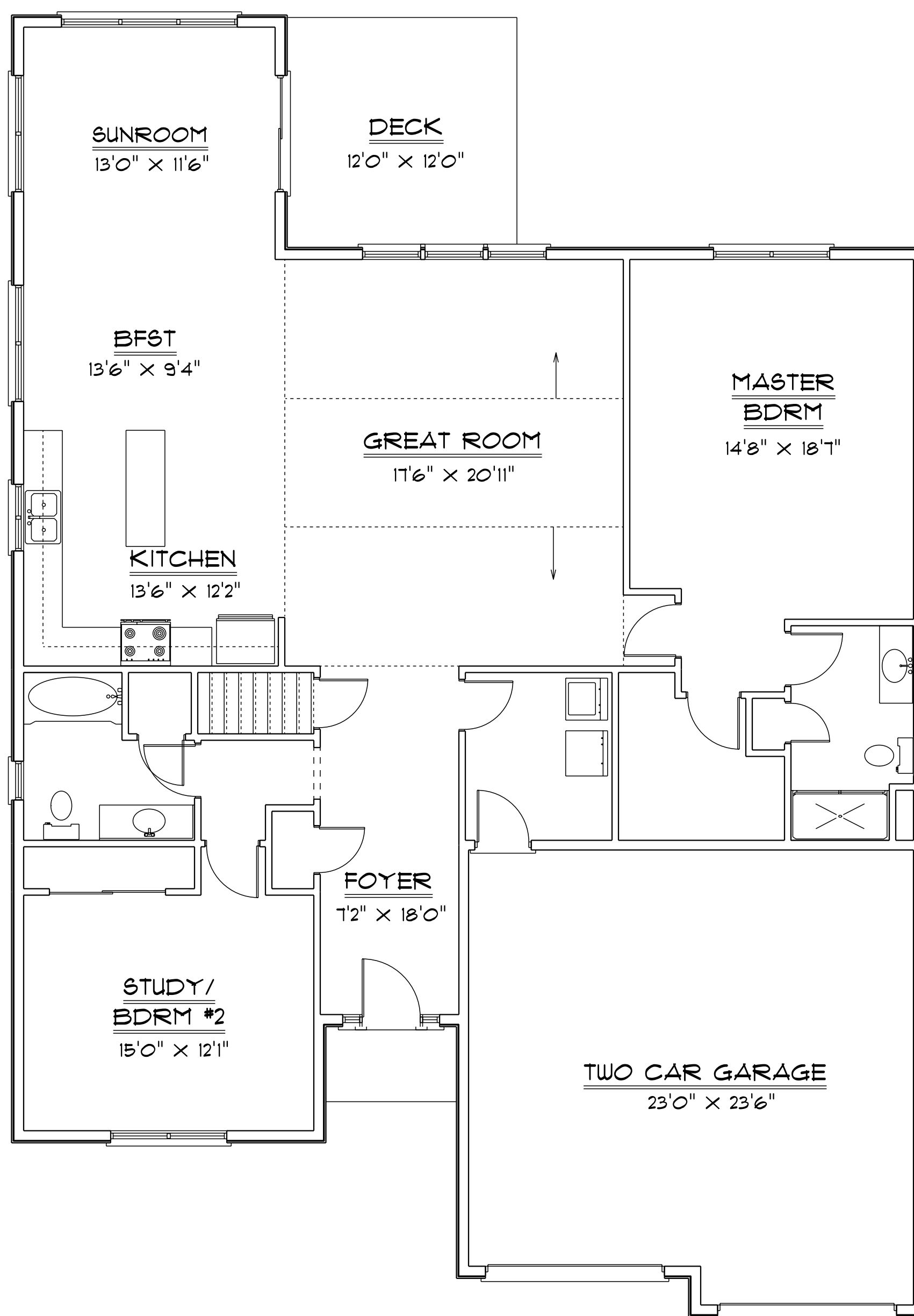
FLOOR PLAN = 1960 S/F (+/-)
